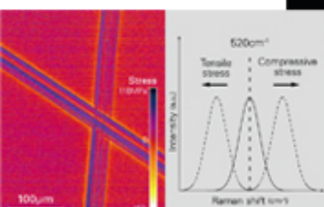
Stress distribution
